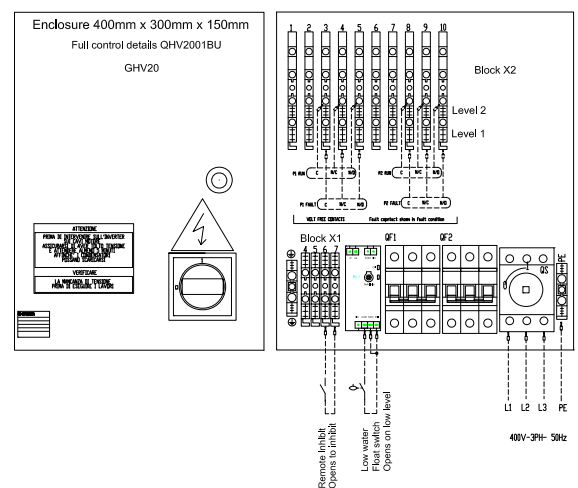
GHV20 three phase booster set 2.2-22Kw
