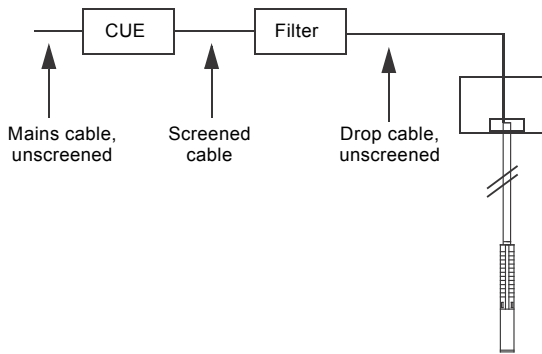
Fig. 22 Example of installation in EMC-insensitive sites
